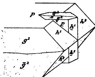
Fig. 4. Macles de Bowling.
