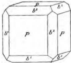
Fig. 4. Fluorine.
